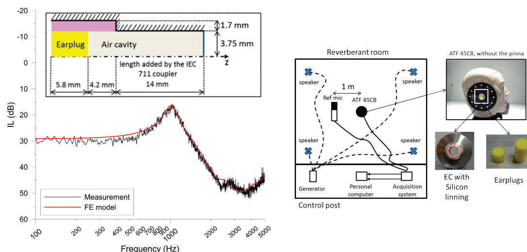
Fig. 2 – Left: comparison of predicted and measured IL for a 5.8mm silicone EP; Right: experimental validation set-up (adapted from (3))
