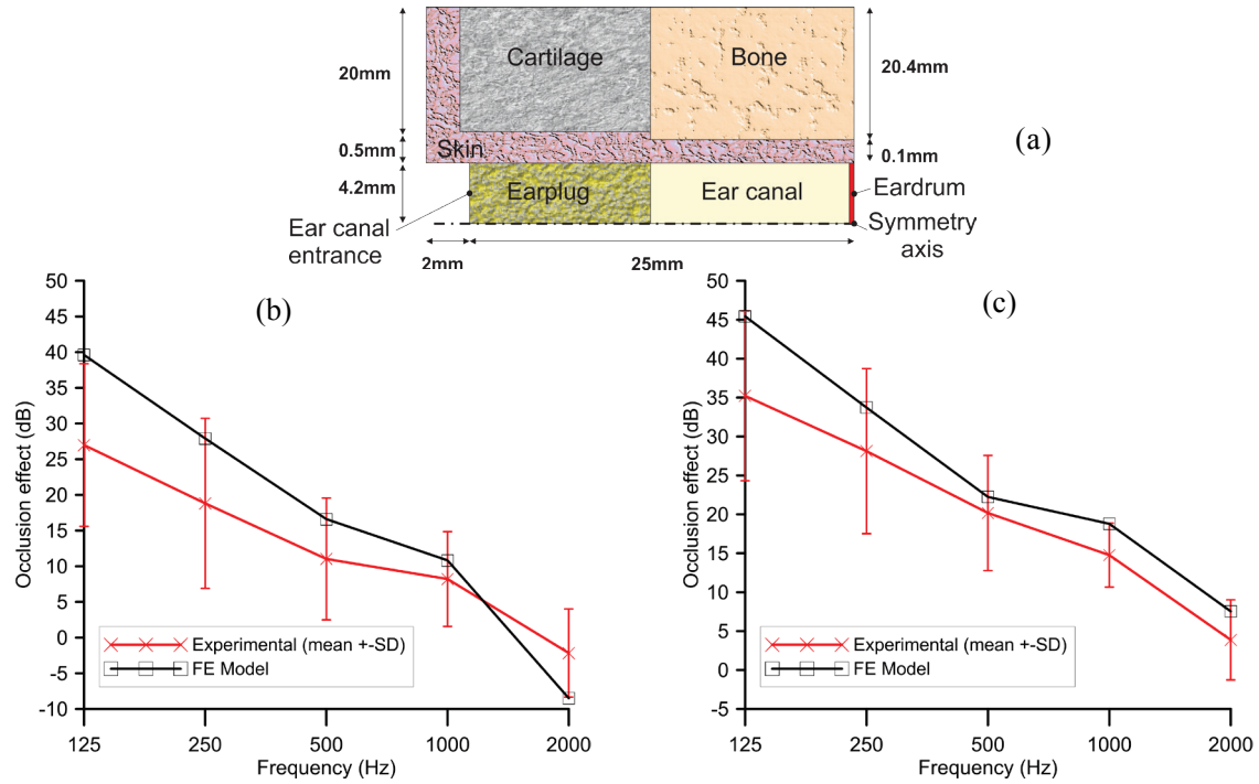
Fig. 4 – Comparison between predicted and measured OE (a) Configuration used in the simulations (b) foam EP (11.1mm insertion depth) (c) silicone EP (11.7mm insertion depth) (adapted from (14))
