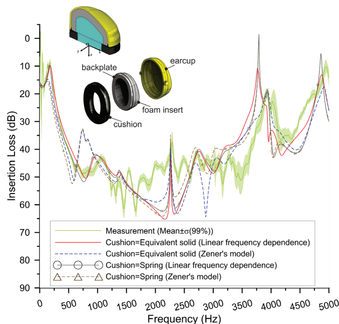
Figure 5 – Comparison between predicted and measured IL for a PELTO-OPTIME 98 earmuff (adapted from (19)).
