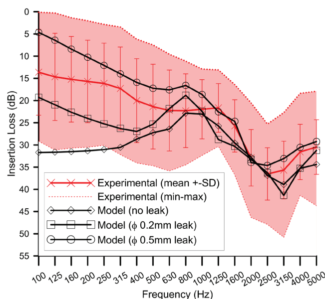
Fig. 3 – Comparison between measured (mean \pm SD) and predicted third octave band IL of a 11.7mm long custom molded EP (no leak, 0.2 mm and 0.5 mm diameter leaks) (adapted from (16)).
