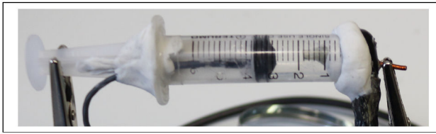
Figure 1. Picture of the measurement tube and probe setup
