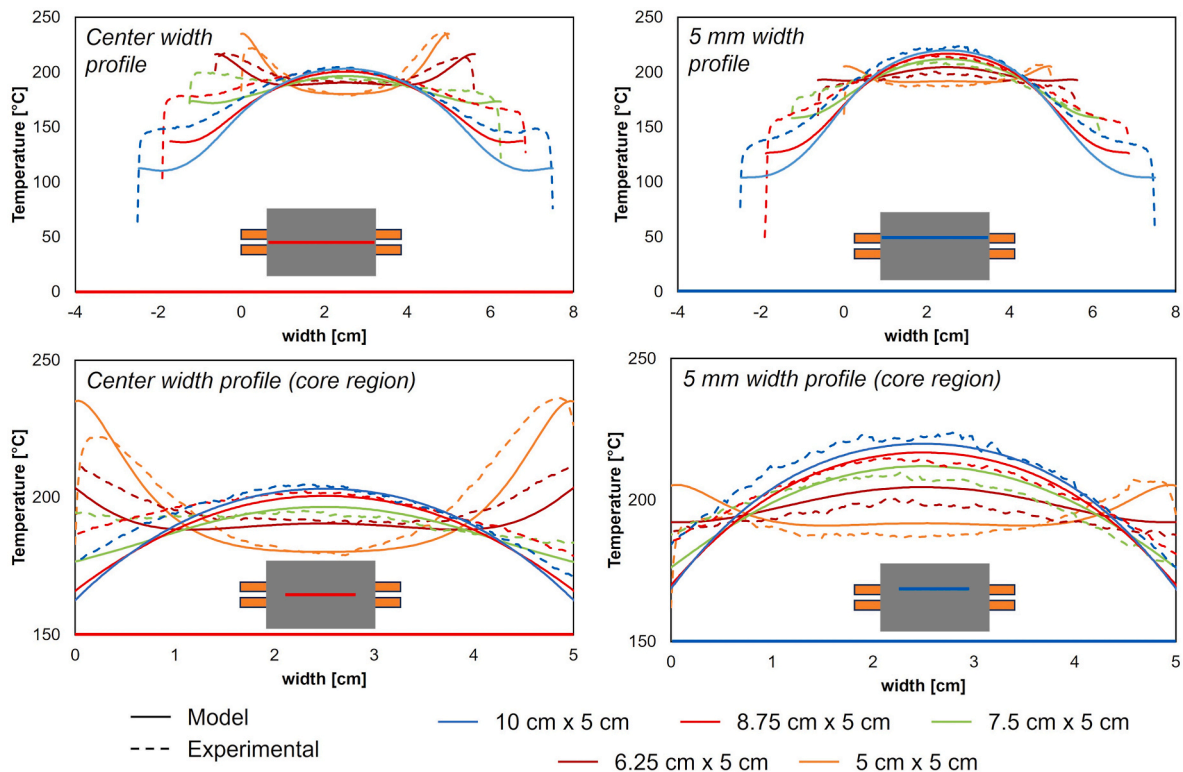
Fig. 11. Induction heating of laminates under 50 A current amplitude for varying sample widths. The temperature distribution along both width profiles is reported. Only the temperature after 90 s is shown for clarity. Experimental measurements (dashed lines) are compared to simulations (solid lines).
