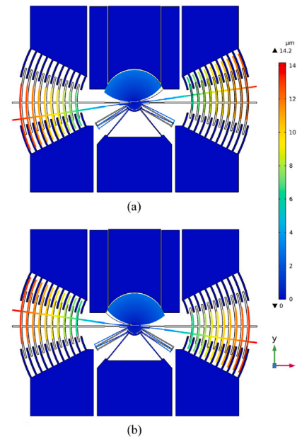
Fig. 5. FEM simulation of the angular displacement of the MEMS structure at an actuation voltage of 150 V: a) CW motion, b) CCW motion.
