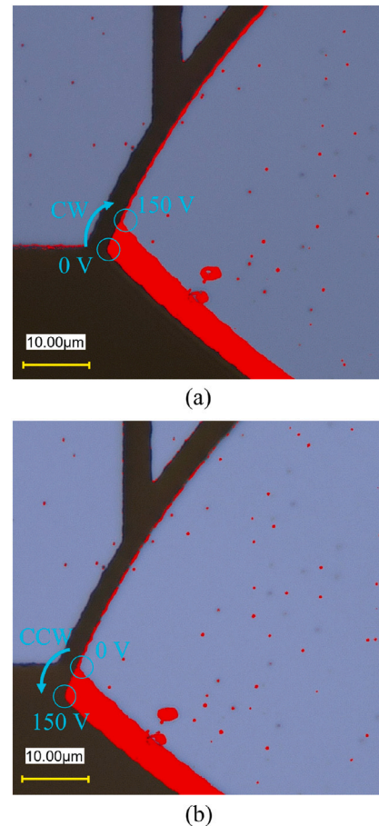
Fig. 8. Processed image output showing the pixel differences between the 0 V and 150 V actuation states. a) CW motion, where the red region corresponds to the initial position at 0 V and the gray region corresponds to the displaced position at 150 V, b) CCW motion, where the gray region corresponds to the initial position at 0 V and the red region corresponds to the displaced position at 150 V. The color inversion reflects the opposite direction of motion (For interpretation of the references to color in this figure legend, the reader is referred to the web version of this article.)
