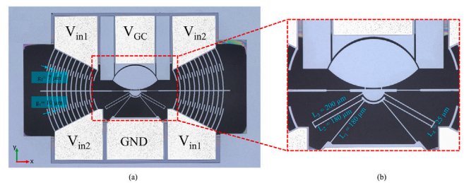
Fig. 1. Fabricated rotary MEMS structure: a) top view, b) zoomed view of the U-shaped spring.
