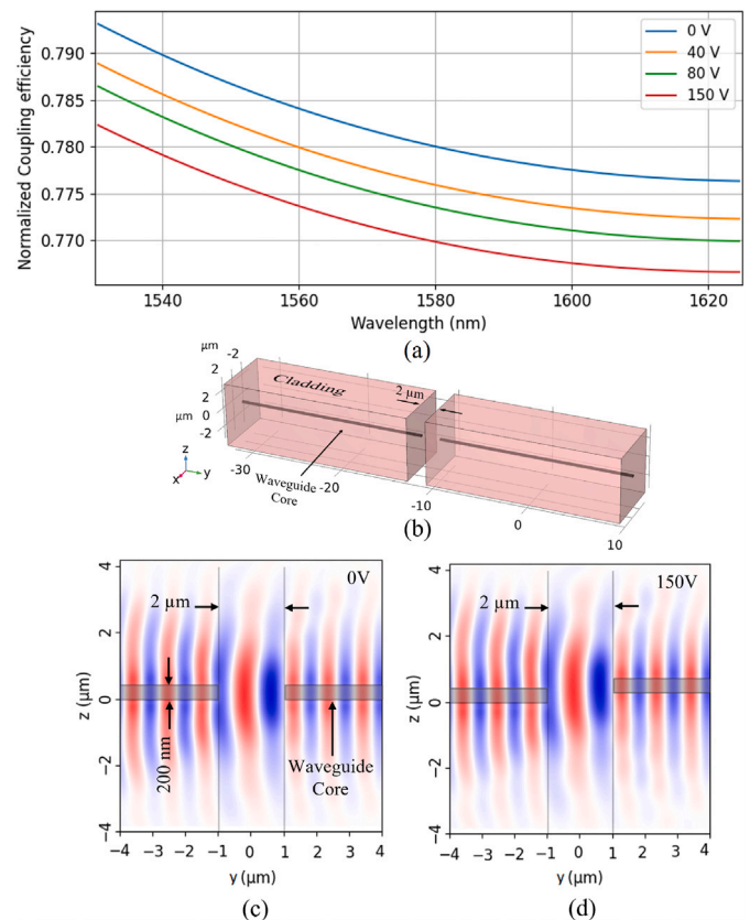
Fig. 7. (a) coupling efficiency from 3D FDTD simulations for actuation voltages ranging from 0 V to 150 V, (b) 3D representation of the simulated waveguide geometry, (c) side view of the simulated optical electric-field distribution at 0 V, indicating the effective 2 \mu\text{m} air gap and the 200 nm-thick SiN waveguide core, and (d) side view of the simulated optical electric-field distribution at 150 V, showing negligible deformation of the optical mode under voltage-induced Z-axis motion.
