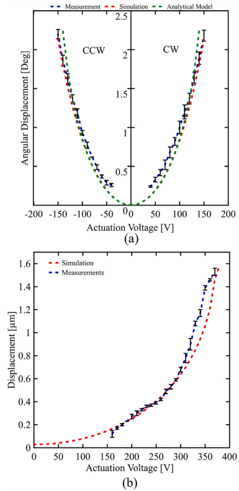
Fig. 10. Measured displacements of the fabricated MEMS structure: a) angular displacement, and b) lateral gap-closing displacement.
