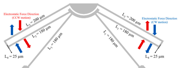
Fig. 2. Simplified schematic of the U-shaped flexure, illustrating the qualitative motion and bending directions under clockwise (CW, blue arrows) and counter-clockwise (CCW, red arrows) electrostatic actuation (For interpretation of the references to color in this figure legend, the reader is referred to the web version of this article.).
