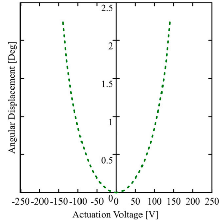
Fig. 3. Plot of the calculated angular displacement versus actuation voltage.
