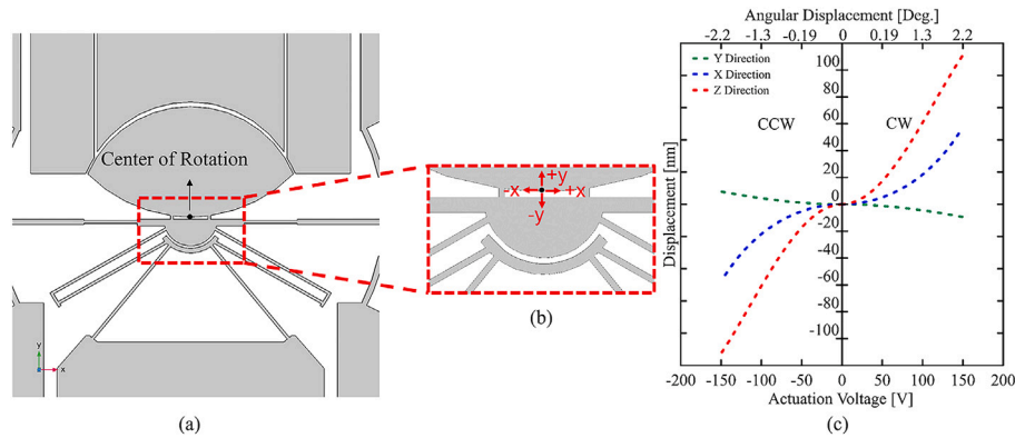
Fig. 6. A) MEMS structure showing the center of rotation, b) Magnified view indicating in-plane X and Y displacement directions, c) simulated translational displacement of the rotation center along the X, Y, and Z axes as a function of actuation voltage (bottom X-axis) for both CW and CCW actuation. The corresponding angular displacement is provided on the top X-axis for reference.
