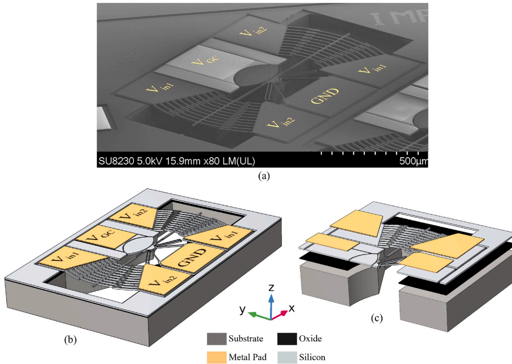
Fig. 4. Fabricated MEMS device: (a) isometric view captured using SEM, (b) 3D view of the layers, and (c) cross Section.
