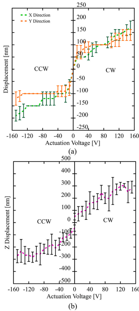
Fig. 9. Measured translational displacement of the center of rotation as a function of actuation voltage during both CW and CCW operation: a) in-plane X and Y displacements, and b) out-of-plane Z displacement. Error bars represent the standard deviation (STD) across five repeated measurements.
