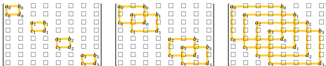
Figure 5: A partial trace applied to an 8 \times 8 matrix, to trace out two qubits, picks out certain elements (labeled a_i, \dots, d_i above) to sum, producing a 2 \times 2 result \begin{bmatrix} A & B \\ C & D \end{bmatrix} where A = \sum_i a_i , ..., D = \sum_i d_i . If the 8 \times 8 matrix is a density matrix \rho_{210} , with rows and columns numbered 0 through 7, then above we see the elements picked out by \text{Tr}_{21}(\rho_{210}) (left), \text{Tr}_{20}(\rho_{210}) (center), and \text{Tr}_{10}(\rho_{210}) (right), where \text{Tr}_{ij} denotes tracing out bits i and j . In other words, the labelings illustrate calls to partialTrace() with qubitsToTraceOut set to [1, 2] (left), [0, 2] (center), [0, 1] (right). Each orange rectangle corresponds to an iteration of the loop at line 53 in the partialTrace() pseudocode, and the subscripts on a_i, \dots, d_i are values of shared_bits . Compare with the patterns in Figure 3.
