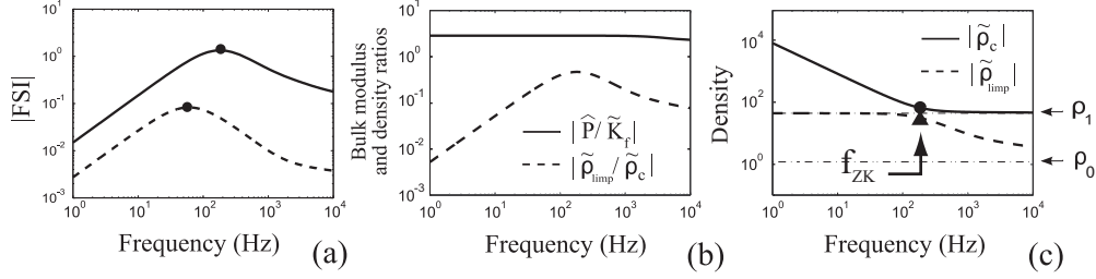
FIG. 1. (a) Parameter FSI for materials (- -) B and (-) C: ( \bullet ) are the approximated values at f_{ZK} (see Eq. (6)); (b) ratio of the characteristic Bulk modulus and moduli of complex densities for material C; (c) moduli of complex densities of the two characteristic waves for material C: ( \blacktriangle ) and ( \bullet ) are the approximated moduli of complex densities at f_{ZK} (see Eq. (4))
