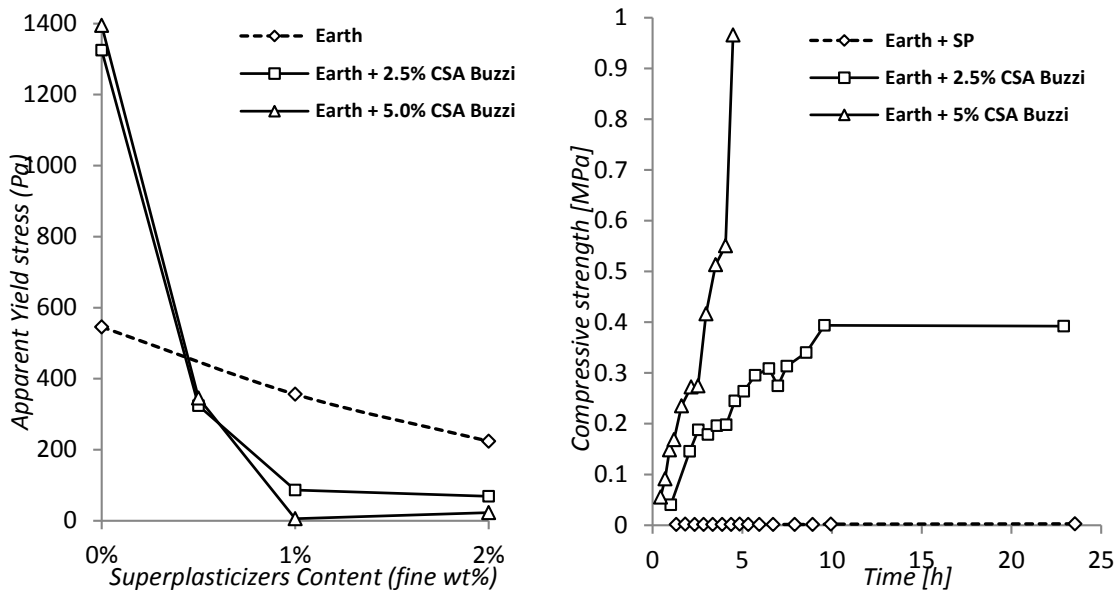
Figure 2: a) effect of SP and CSA cement on earth with 55% of fine particles and b) early development of compressive strength over time measured by penetrometer
