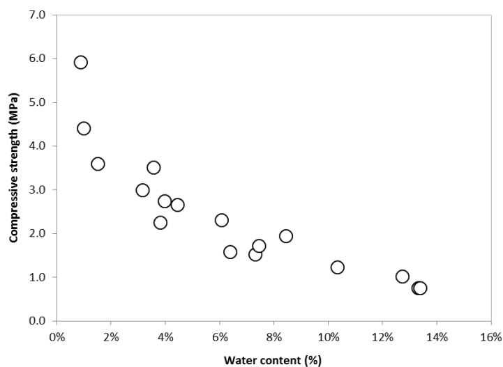
Figure 3: Compressive strength as a function of water content in sample. (5% CSA and 1% PCE)
